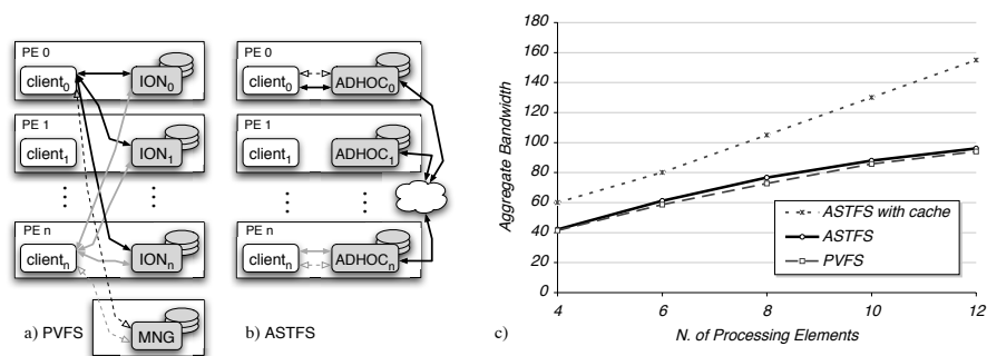
Figure 5: a) Many clients accessing a PVFS. Each PE hosts a client is required to be a ION. Solid edges show data paths, dashed edges meta-data paths. b) Many clients accessing a ASTFS. c) Comparison among PVFS and ASTFS. Each client read a partition of the file in segments of 10MB randomly chosen within its partition. In both cases, each client reads the same 800MByte file spread among all PEs.
